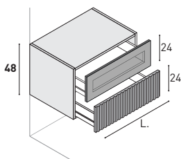
Base unit 1 upper jumbo metal drawer with black aluminium frame + Stop-sol glass, 1 lower jumbo metal drawer.
