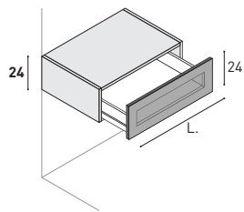
Base unit 1 jumbo metal drawer with black aluminium frame + Stop-sol glass.
