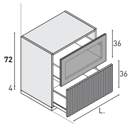
Base unit 1 upper jumbo metal drawer with black aluminium frame + Stop-sol glass, 1 lower jumbo metal drawer.
