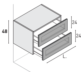
Base unit 2 jumbo metal drawers with black aluminium frame + Stop-sol glass.
