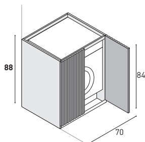
Base unit 2 doors for washing machine, pull-out plinth.
