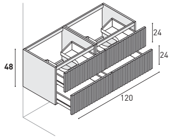
Uniblock 4 jumbo metal drawers.
