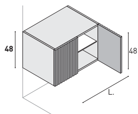
Base unit 2 doors, 1 glass shelf.
