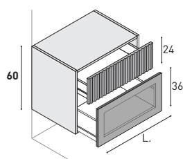
Base unit 1 upper jumbo metal drawer, 1 lower jumbo metal drawer with black aluminium frame + Stop-sol glass.
