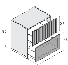
Base unit 1 upper jumbo metal drawer, 1 lower jumbo metal drawer with black aluminium frame + Stop-sol glass.
