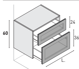
Base unit 2 jumbo metal drawers with black aluminium frame + Stop-sol glass.
