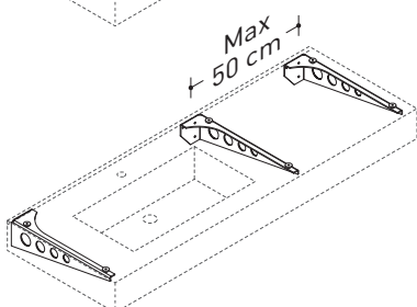
2 Brackets + 1 Side bracket each 50 cm
