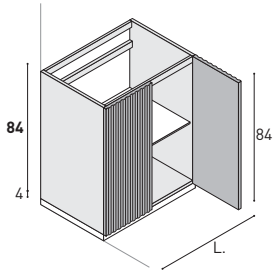
Washbasin unit 2 doors, 1 glass shelf.
